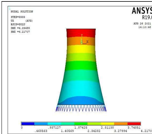
Fig. 11. Maximum Displacement of fixed base CT-1 for 200mm Thickness
